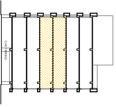
Option II Section showing Unit of 11000 sqft spread over 2 floors
